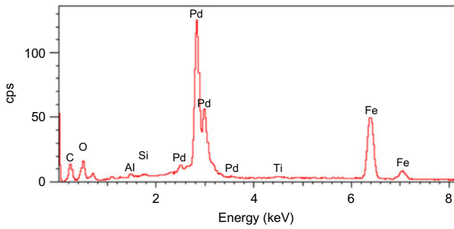
Fig. 3. EDS result of \text{Fe}_x\text{Pd}_{100-x} nanoparticles with x = 60 .
