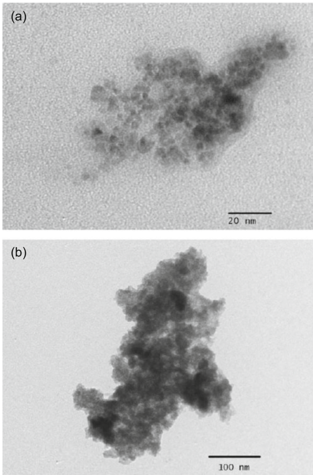
Fig. 1. TEM images of as-prepared (a) and annealed (b) \text{Fe}_{60}\text{Pd}_{40} nanoparticles.
