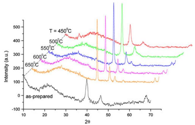
Fig. 2. X-ray patterns of as-prepared and annealed \text{Fe}_{60}\text{Pd}_{40} nanoparticles.
