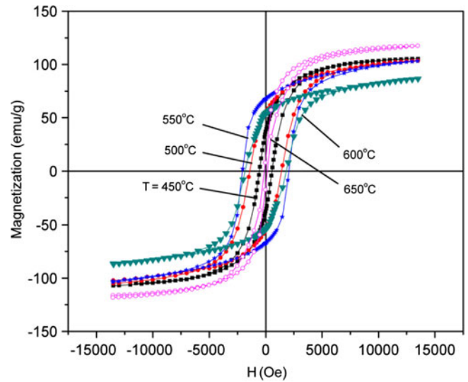
Fig. 5. Room temperature magnetization curves of \text{Fe}_{60}\text{Pd}_{40} nanoparticles annealed at various temperatures.
