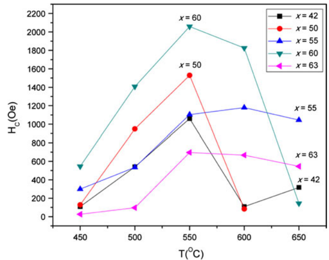
Fig. 6. The annealing-temperature dependence of coercivity of the \text{Fe}_x\text{Pd}_{100-x} nanoparticles.
