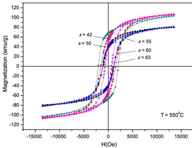
Fig. 4. Room temperature magnetization curves of \text{Fe}_x\text{Pd}_{100-x} nanoparticles annealed at 550\text{ }^\circ\text{C} with various x .
